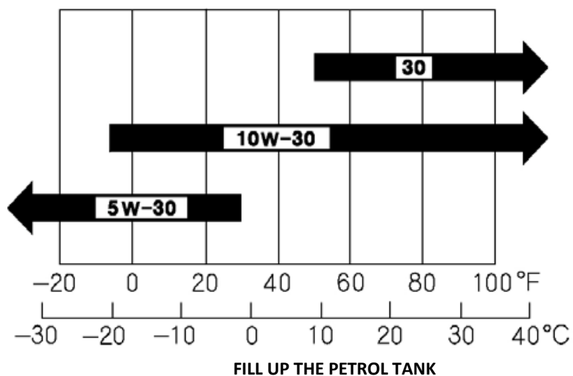
SAE Viscosity Grades
